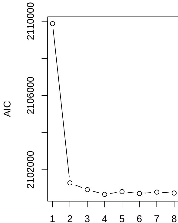
AIC
